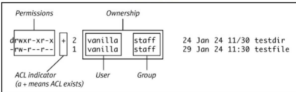
Figure 8.8. Diagram showing which parts of the listing are the permissions and which parts are the ownership information.
